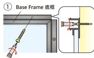
① Base Frame 底框 Fix the base frame with screws on the wall first. 先將底框以螺絲安裝至牆上
