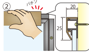
② Put the ABS frame on top of base frame, and push down until hear a "Ba" sound 將樹脂邊框放於底框上按下直至聽到“啲”一聲
