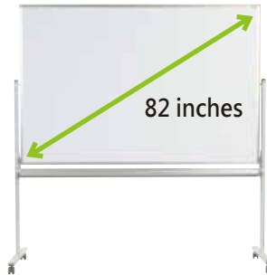
UM46T / UM46TD External Dimensions / W1926×D610×H1990 Outer Dimensions / W1810×H1210 Board Dimensions / W1770×H1170
